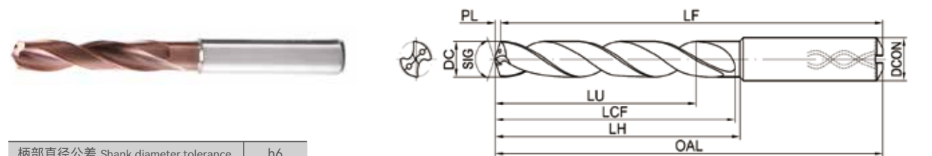
内冷钻头 internal coolant design
